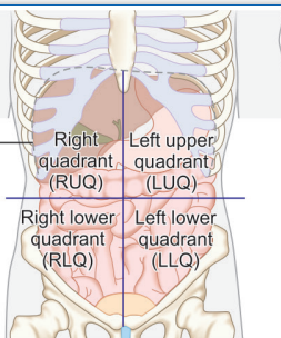
Abdominopelvic quadrants
