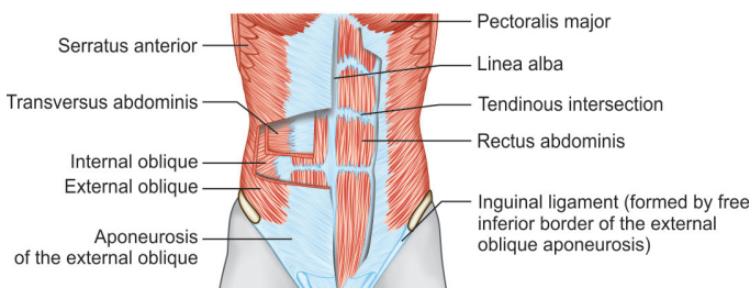
Abdominal muscles
