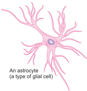
Astrocyte
