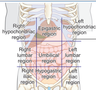
Abdominopelvic regions
