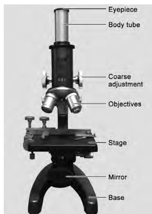
Fig. 1.1: Monocular compound microscope (front view)
