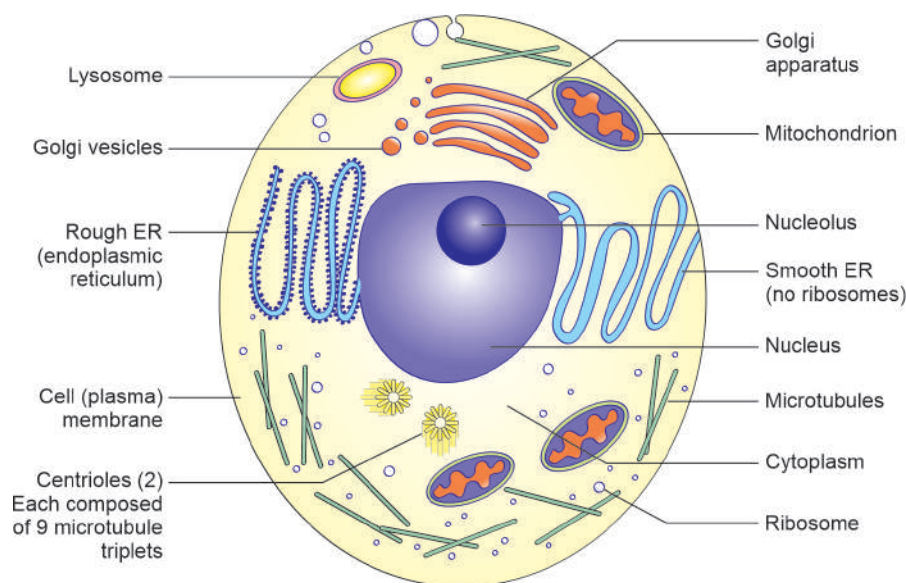
Fig. 1.1: Eukaryotic cell
